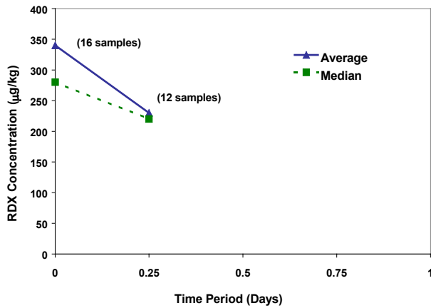
Figure 1. Chemical oxidation results, washed soils - Brice/UNL
