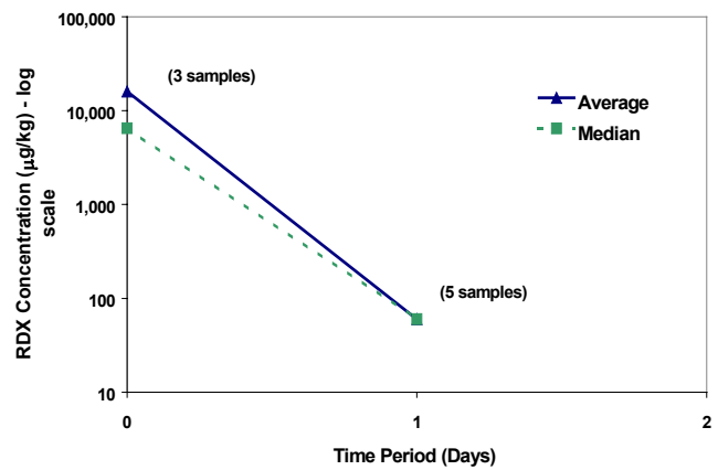
Figure 3. Low temperature thermal destruction results, untreated soils - TerraTherm
