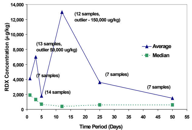
Figure 4. Composting results, untreated soils - BSI
