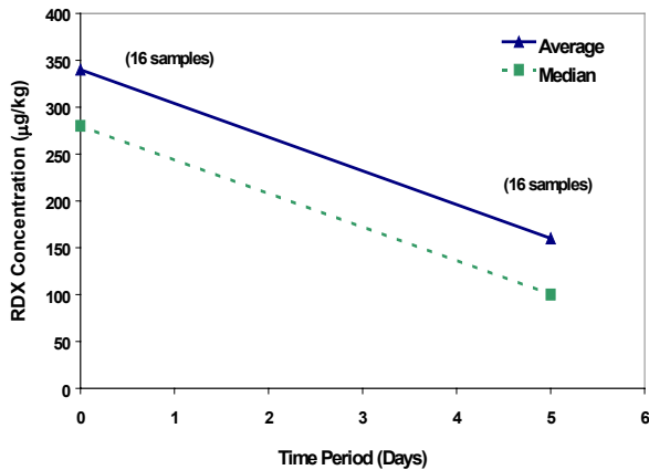
Figure 2. Post treatment chemical reduction results, washed soils - Brice/UNL
