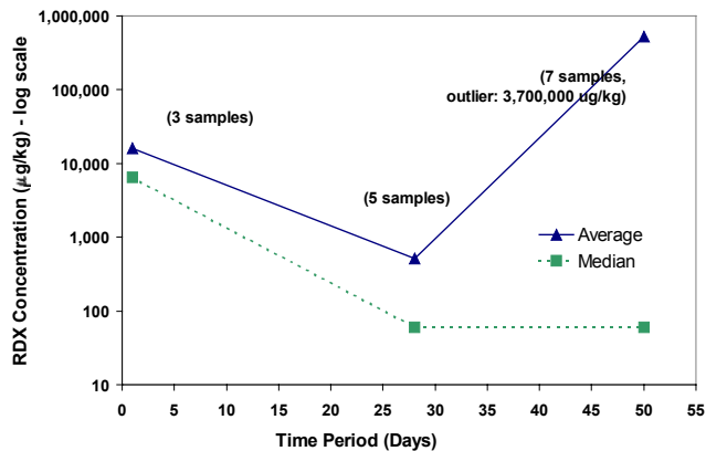
Figure 5. Solid phase bioremediation results, untreated soils - Grace Canada
