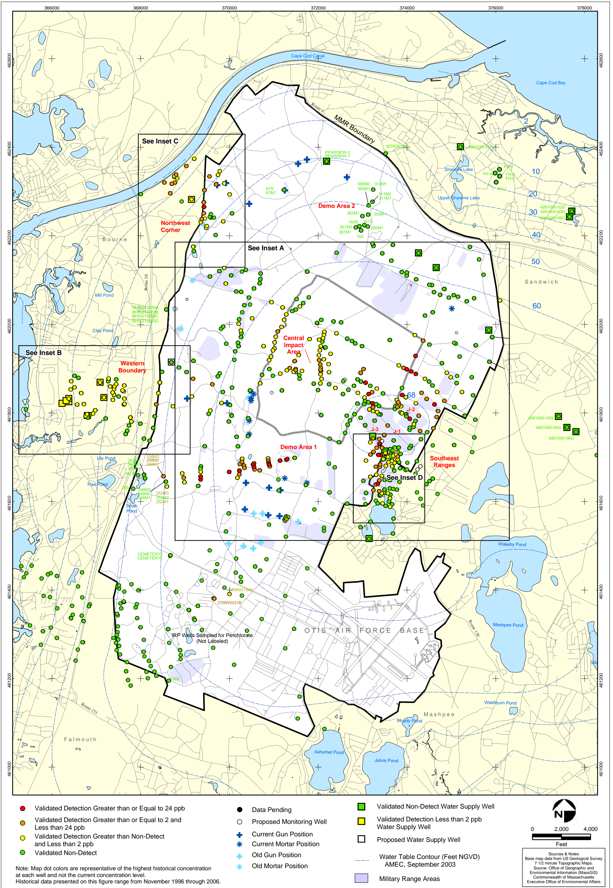
Perchlorate in Groundwater Compared to a 2 ppb Concentration Validated Data as of 11/22/06
