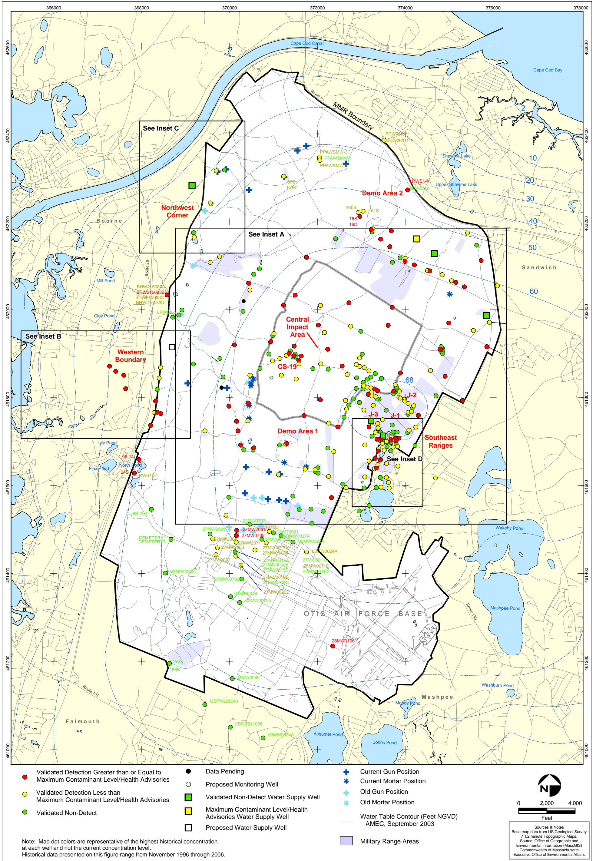
BEHP in Groundwater Compared to a 4 ppb Concentration Validated Data as of 12/29/06
